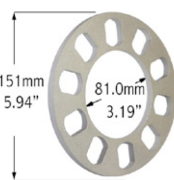
5mm (1/4") Thick
