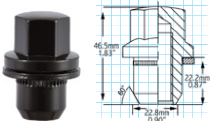
Range Rover - (7/8")
