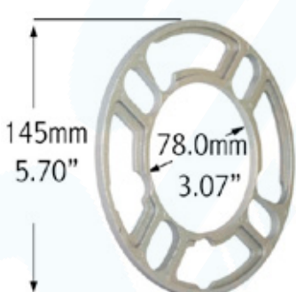
5mm (1/4") Thick
