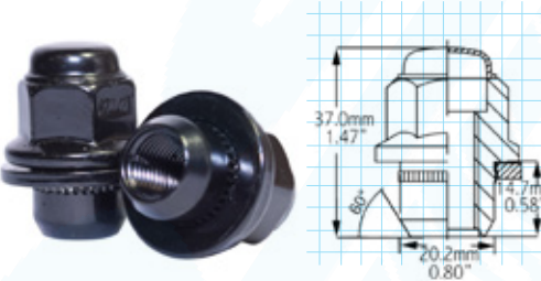
Toyota/Nissan - (13/16")
