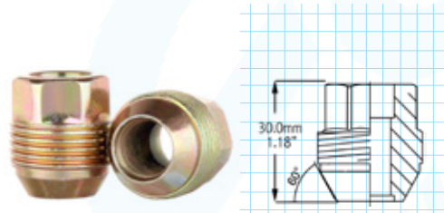
Chevrolet - (7/8")
