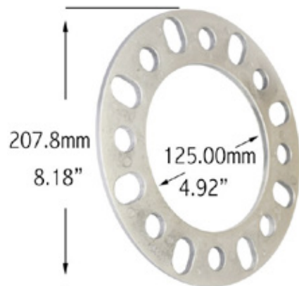
6mm (1/4") Thick
