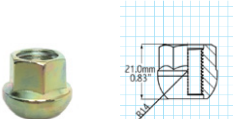
Porsche Open-End (3/4")
