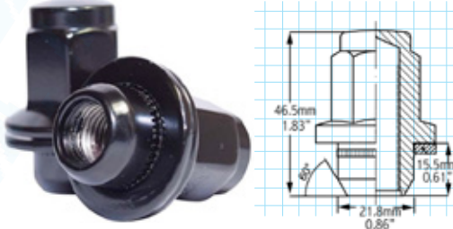
Toyota Tundra (7/8")
