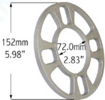
8mm (5/16") Thick
