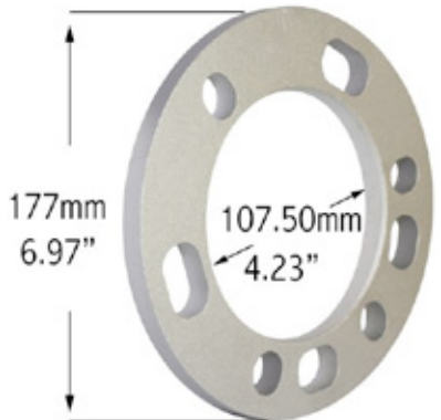
12mm (1/2") Thick
