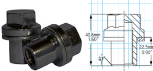
Range Rover - (7/8")
