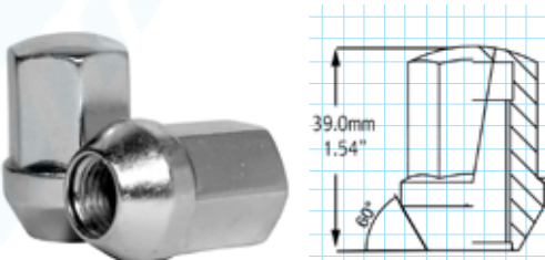
Chrysler/Chevrolet (7/8")
