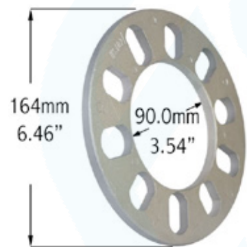
8mm (5/16") Thick
