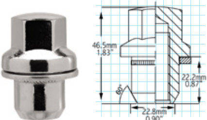
Range Rover - (7/8")
