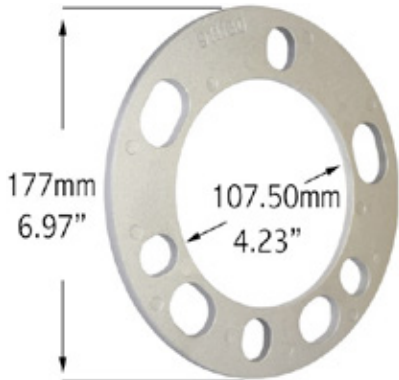
6mm (1/4") Thick
